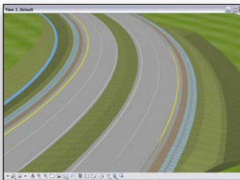
Provides divided highway design with independent horizontal and vertical control.
