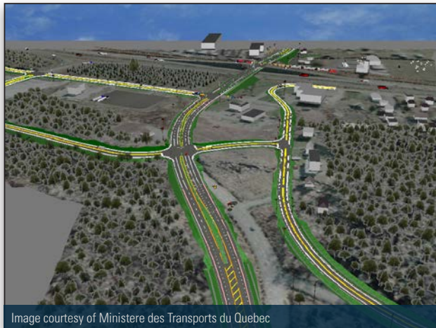
Reshaping of the Route 20 freeway at the Route 171 interchange in Quebec City.
