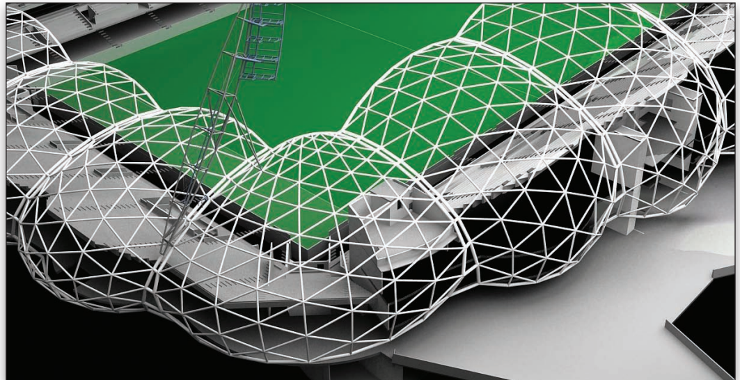
Image of a model designed with Structural Modeler and GenerativeComponents
